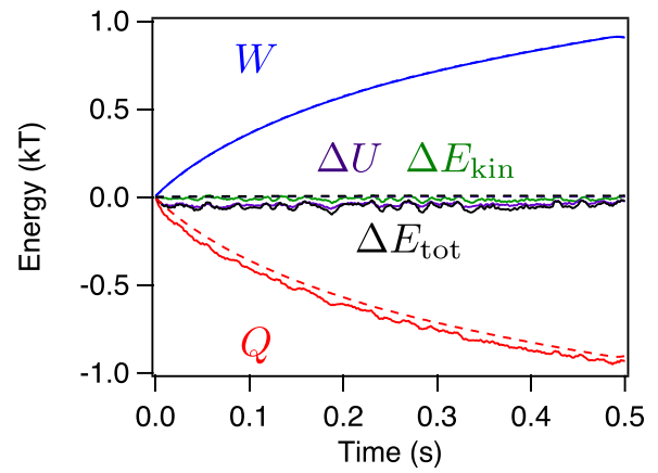
FIG. 4. The same as Fig. 3, but for the isothermal process, where \kappa changes linearly with time from (5.0 \pm 0.2) pN/ \mu\text{m} to (32.0 \pm 0.2) pN/ \mu\text{m} at constant T_{\text{kin}} = T .
